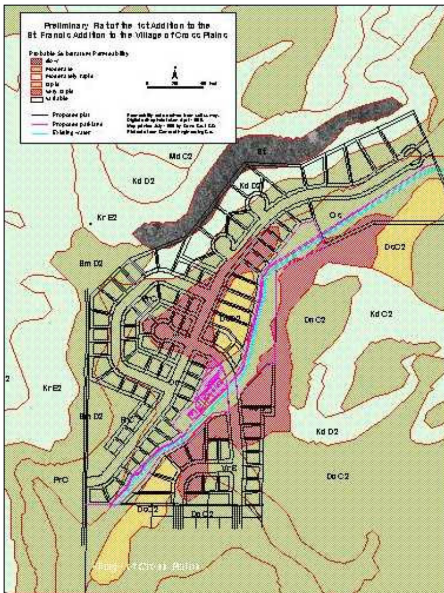
Figure 1.4-1 St. Francis Addition Permeability Analysis
