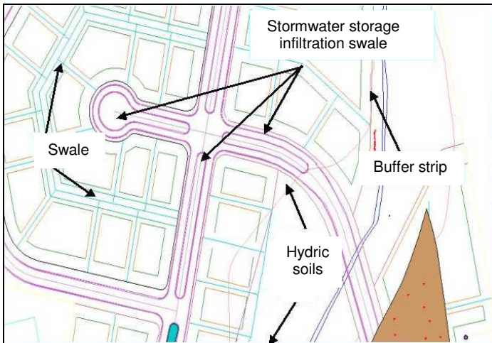
Figure 1.4-2 Detail from St. Francis Addition Plan
